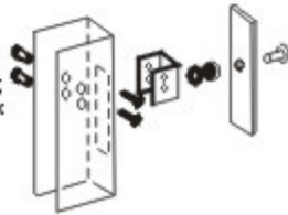
Flush Bonding Magnetic Lock
